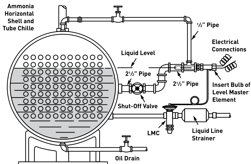
Figure 4: Typical Installation
