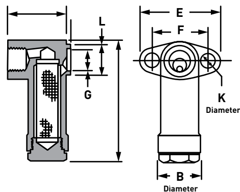
Dimensional Diagram: “XD” Strainer
