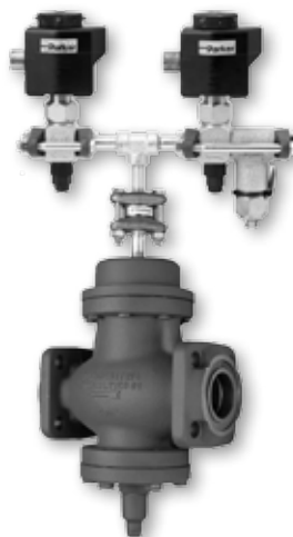
S9A with S9 Pilot Assembly
