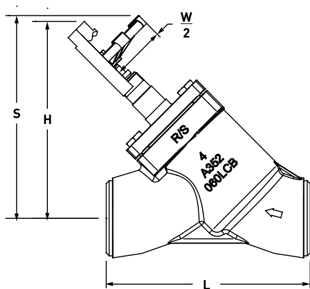
Dimensional Diagram: WN Globe “Y” Body
