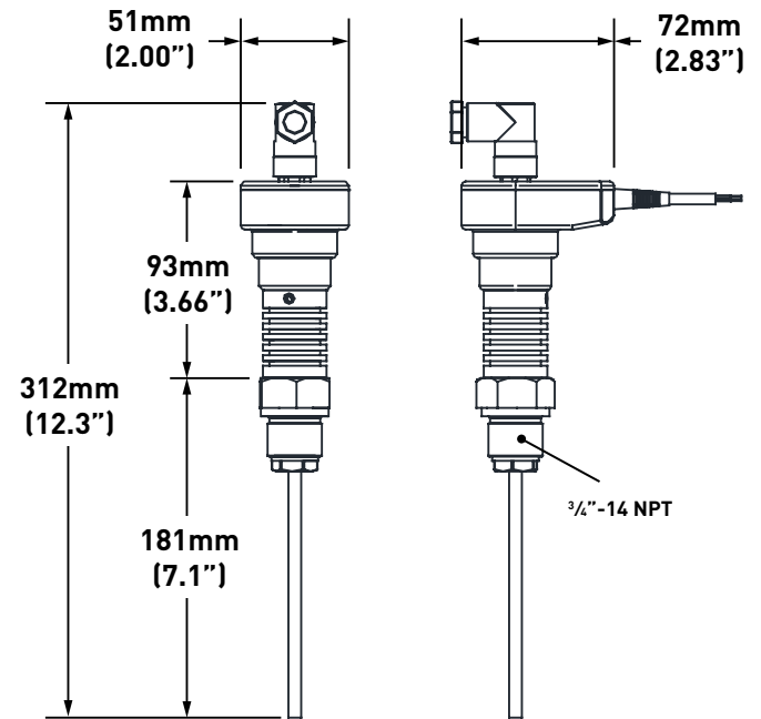
Dimensional Diagram: Liquid Level Control Sensor (HBLC)
