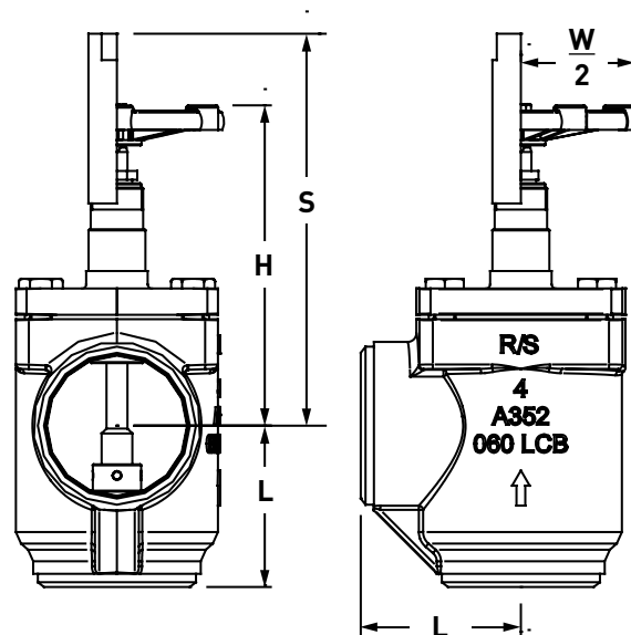
Dimensional Diagram: WN Angle Body
