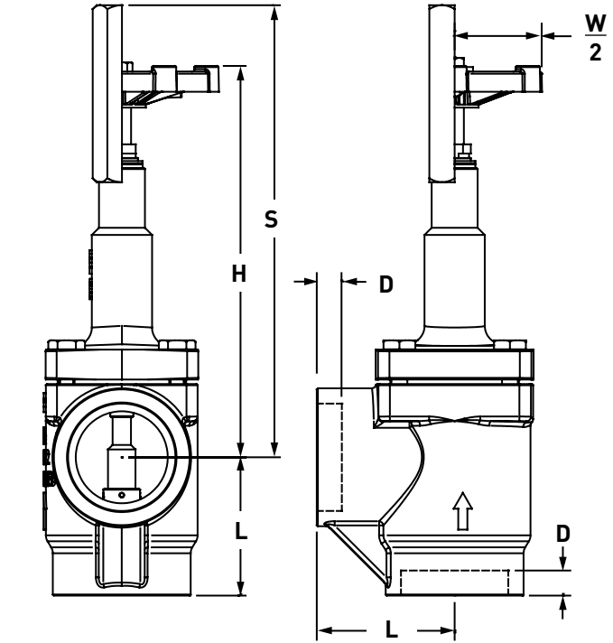
Dimensional Diagram: SW Extended Bonnet Angle Body
