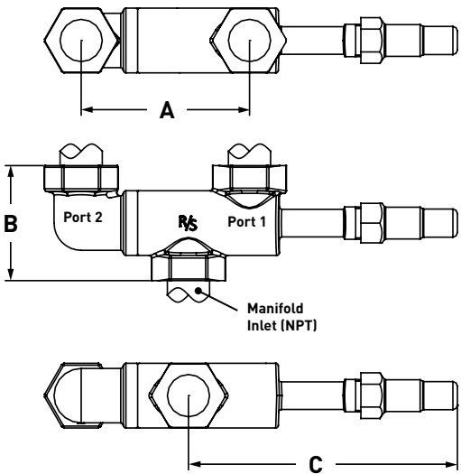
Dimensional Diagram: M1 Dual SR/SRH Safety Relief Valve Manifold
