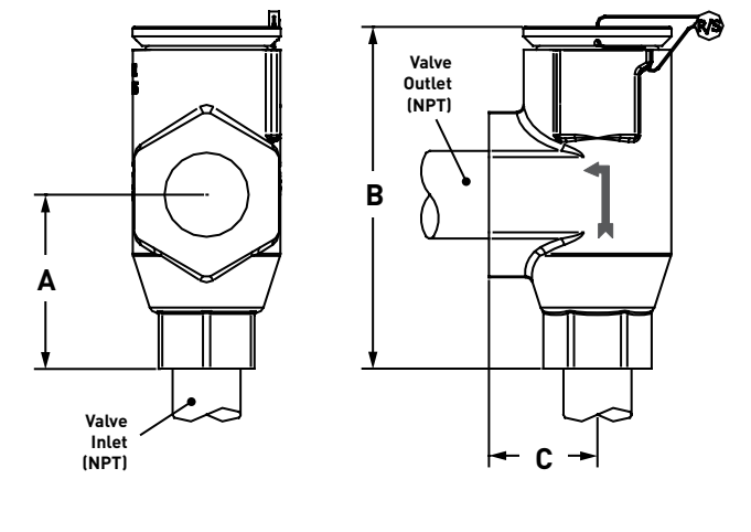
Dimensional Diagram: SR/SRL Series Safety Relief Valve (Single)
