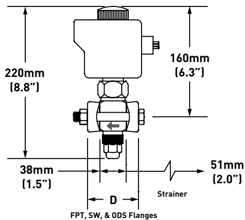
Dimensional Diagram: S6N, S8F Solenoid Valves
