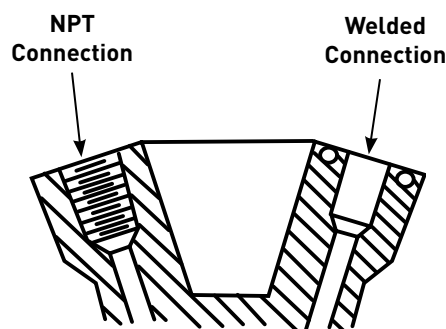
Either NPT connection or welded connections of steel body distributors
