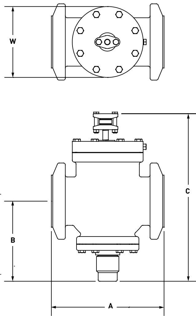
Dimensional Diagram: CK-2 Gas Powered Suction Stop Valves
