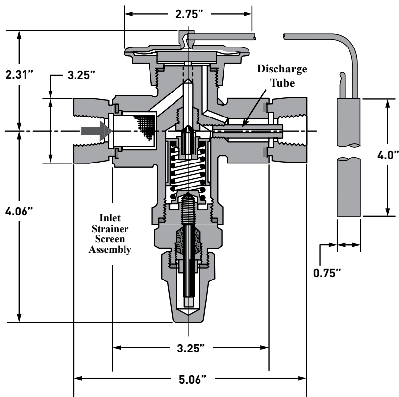
Dimensional Diagram: Type D Thermostatic Expansion Valves
