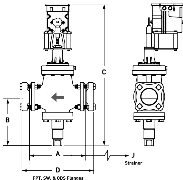
Dimensional Diagram: A4AM, OM Electrically Compensated Pressure Regulator
