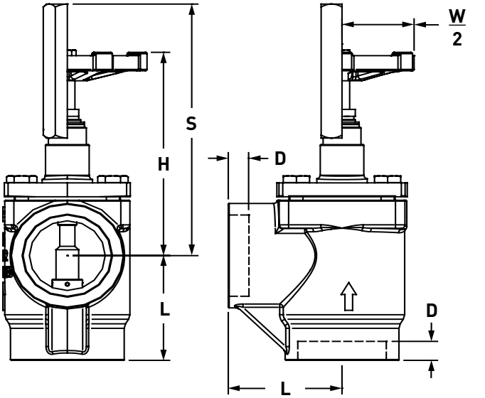
Dimensional Diagram: SW Angle Body
