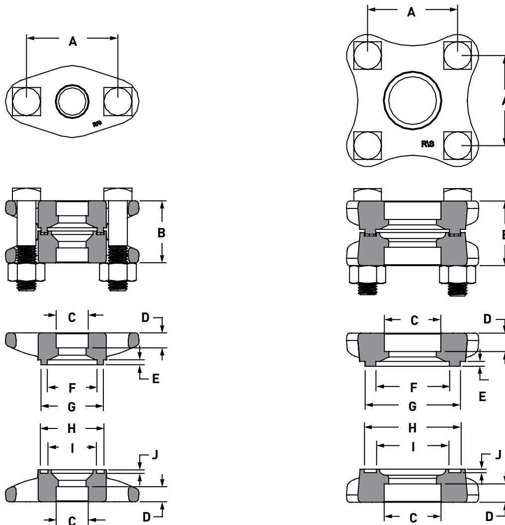
Dimensional Diagram: Socket Weld (SW) Flanges
