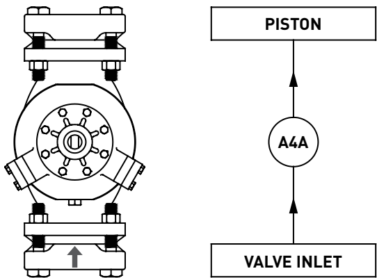
Flow Diagram: A4_Z Inlet Pressure Regulator
