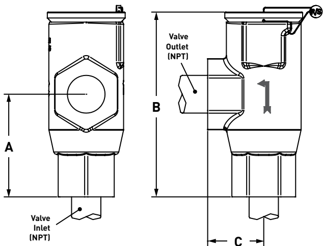
Dimensional Diagram: SRH Series Safety Relief Valve (Single)
