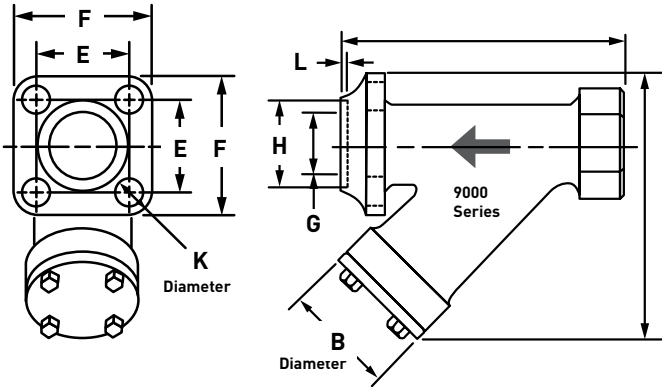
Dimensional Diagram: 8000 Series Strainer
