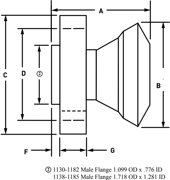
Dimensional Diagram: 1130, 1182, 1138 and 1185 Ammonia Distributors
