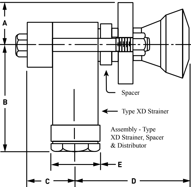
Dimensional Diagram: Aluminum Flange No. 207651 for Type 1180 Distributor
