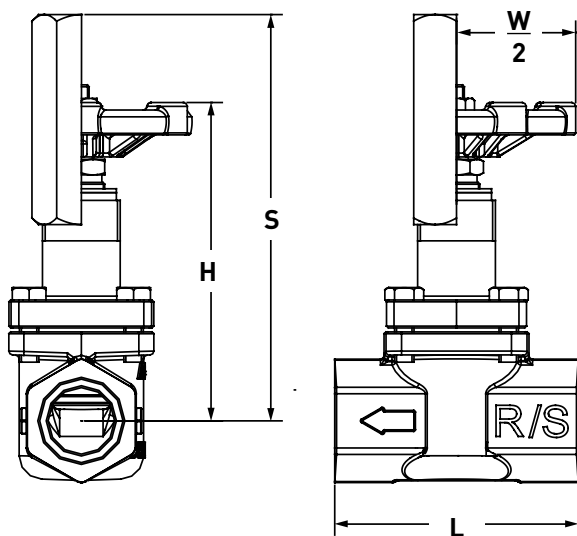
Dimensional Diagram: FPT Globe "T" Body
