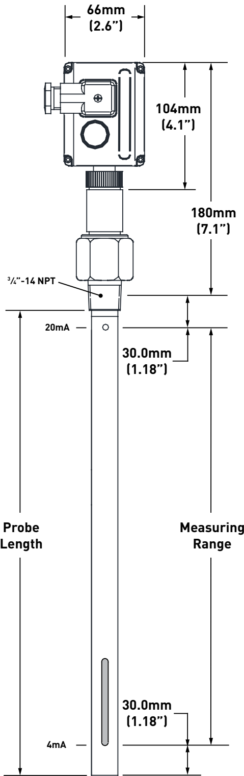
Dimensional Diagram: Liquid Level Transmitter (HBLT-A1)
