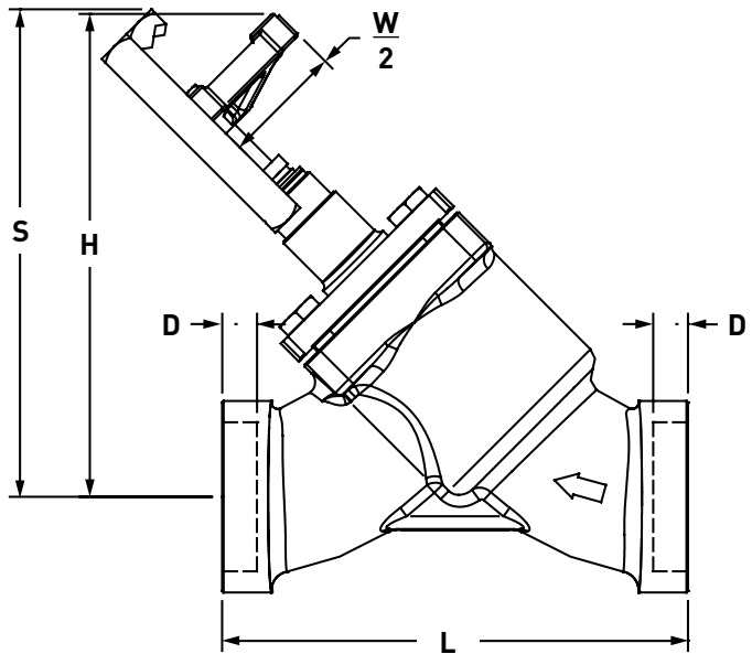
Dimensional Diagram: SW Globe “Y” Body
