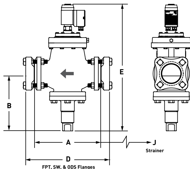
Dimensional Diagram: A4AJ Electric Pilot Pressure Regulator
