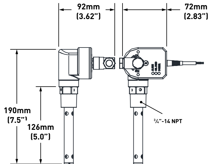
Dimensional Diagram: Oil Level Control Sensor (HBOC)
