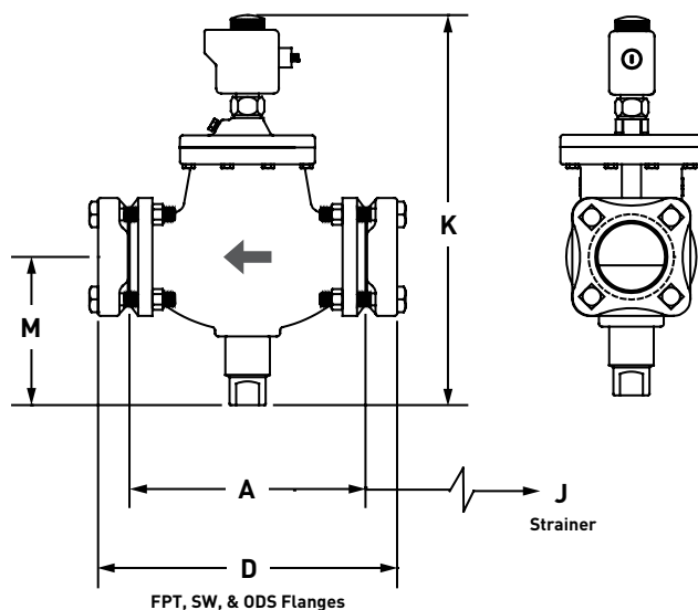
Dimensional Diagram: S5A Solenoid Valves
