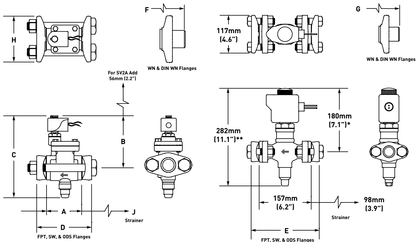
Dimensional Diagram: SV2 Solenoid Valves
