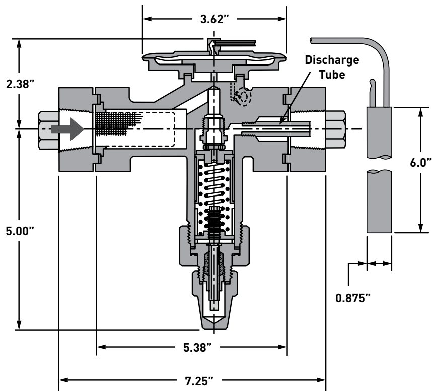
Dimensional Diagram: Type A Thermostatic Expansion Valves
