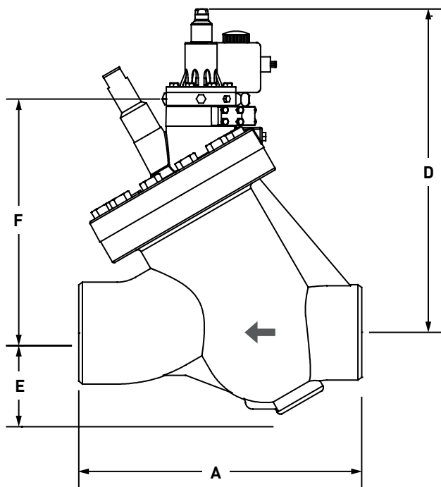
Dimensional Diagram: A4WOES Outlet Pressure Regulator
