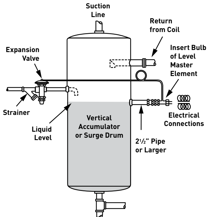
Figure 2: Typical Installation
