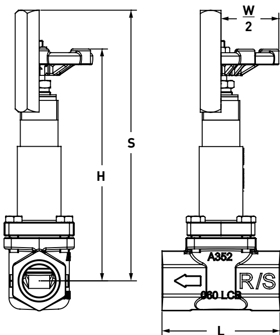
Dimensional Diagram: FPT Extended Bonnet Globe "T" Body
