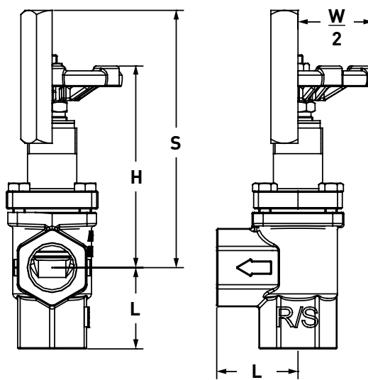
Dimensional Diagram: FPT Angle Body
