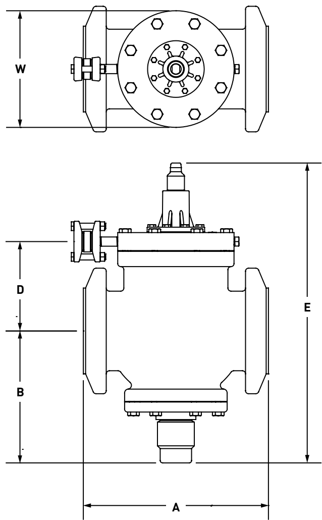
Dimensional Diagram: CK-5 Gas Powered Suction Stop Valves
